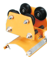
Model No. CE - 31 Four Wheel Cable Clamping Dia : 38mm to 75mm (Round - Flat Cable)
