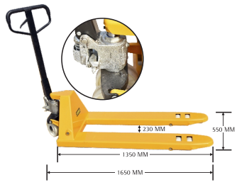
HAND PALLET TRUCK
